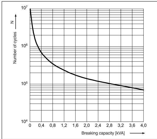
Electrical life at AC resistive load
