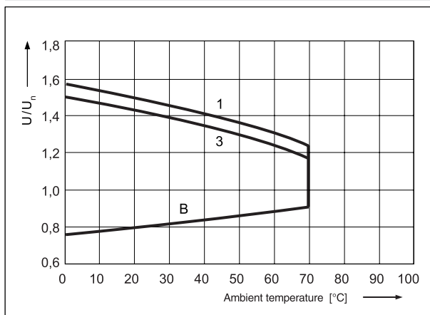
Coil operating range - DC
