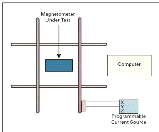
The CXM113 is Calibrated Using a Precision 3-axis Helmholtz Coil
